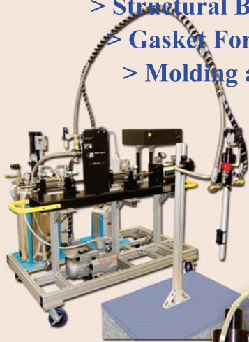
Portable Cart Remote Mixer Vacuum Pump
