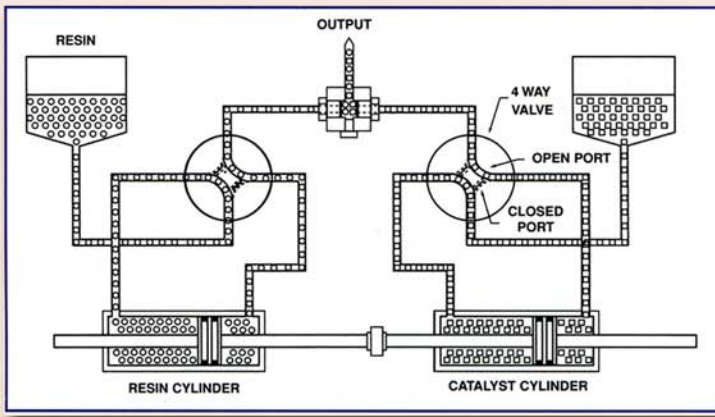
2500 Double Acting Flow Schematic
